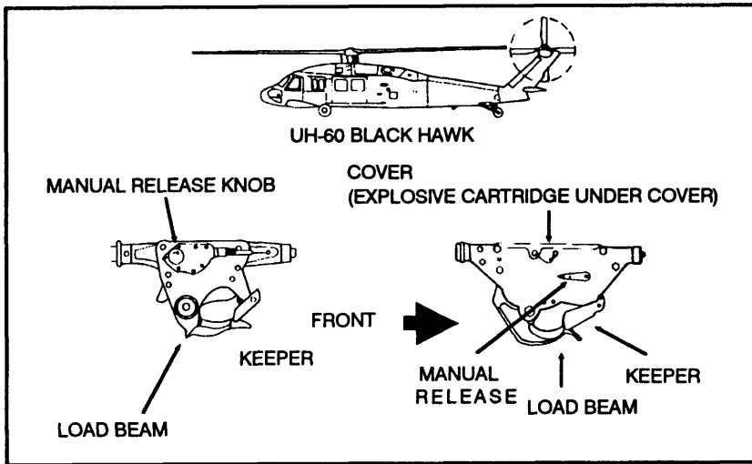
Figure 5-9. UH-60 Black Hawk and its cargo hooks.
