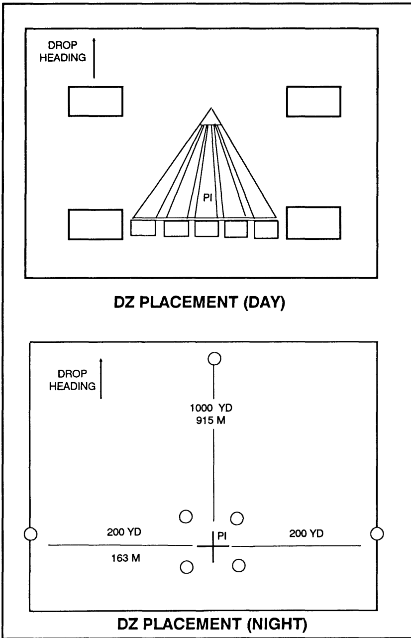
Figure 6-11. Drop zone placement.
