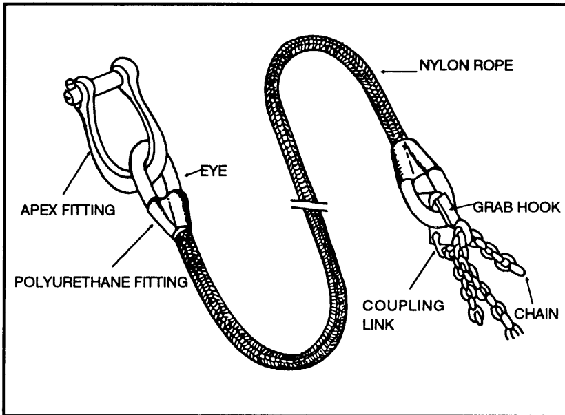
Figure 5-4. 10,000-pound capacity sling set.
