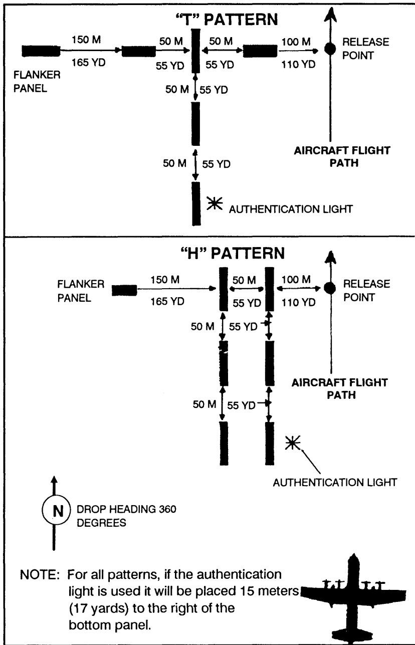
Figure 6-4. Panel emplacement.
