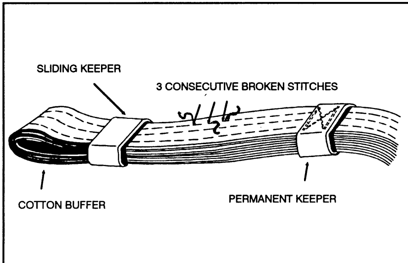
Figure 5-2. Unserviceable slings.
