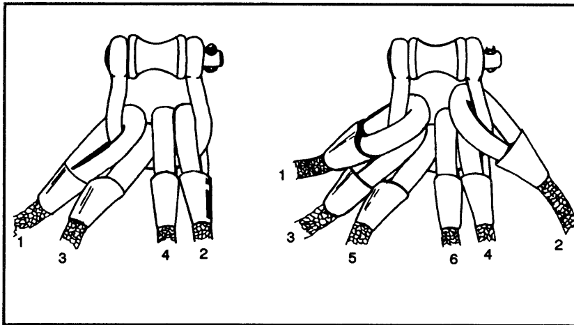
Figure 5-6. Sling leg numbering sequence.
