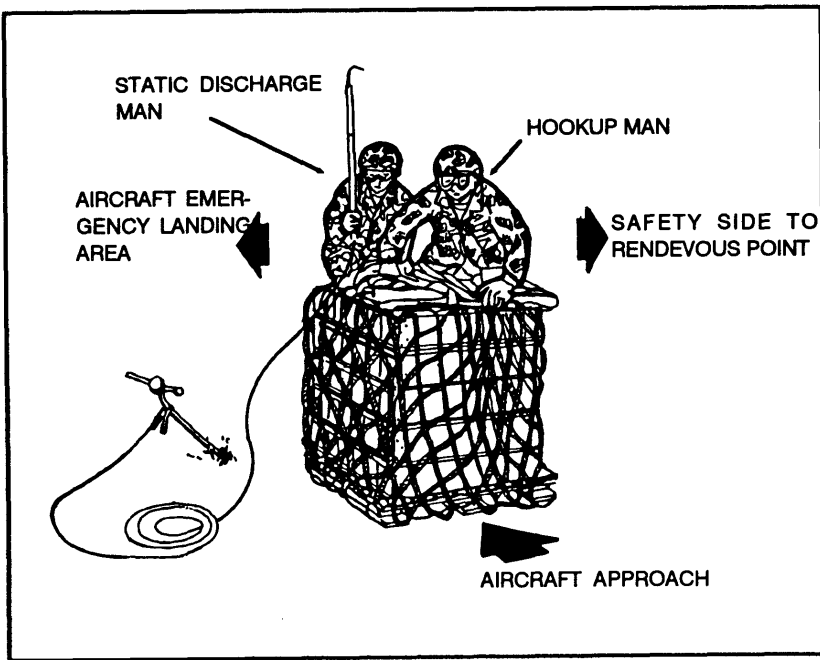
Figure 5-15. Hookup team's position.
