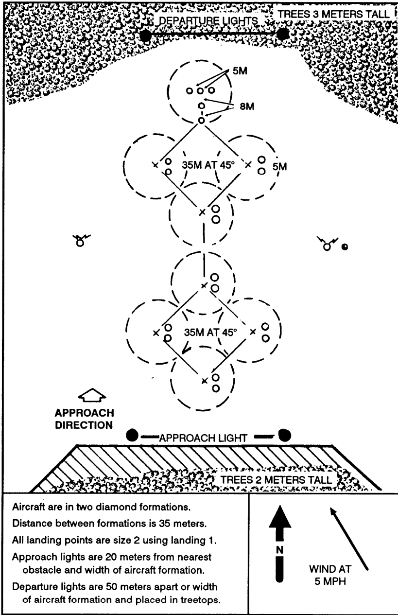
Figure 4-9. Utility helicopter night landing site, diamond formations.
