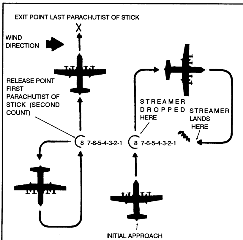
Figure 6-7. Wind streamer vector count.
