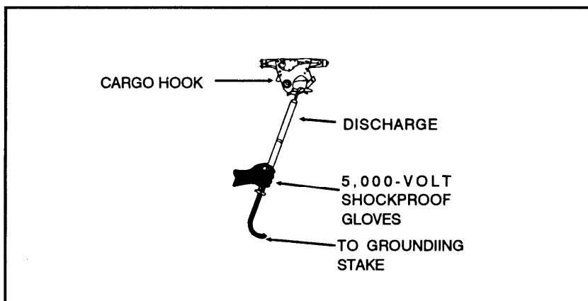
Figure 5-14. Grounding technique.
