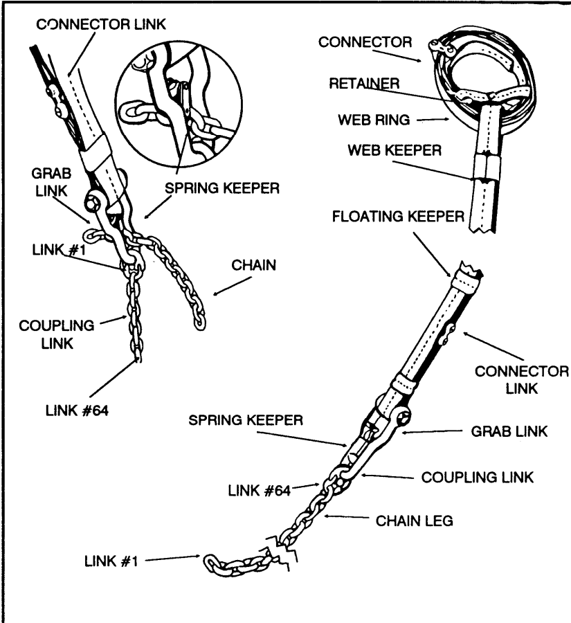
Figure 5-3. Parts of the multi-leg sling set.
