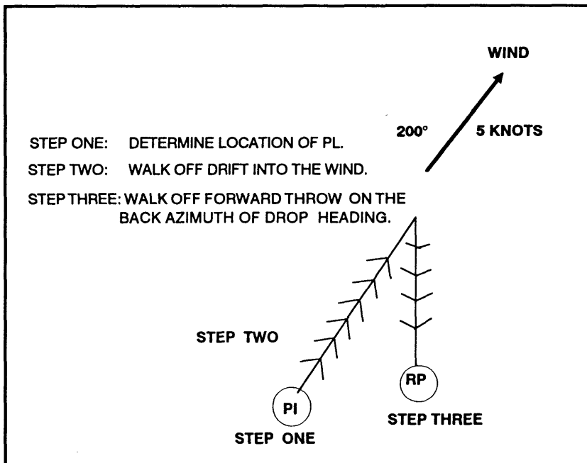
Figure 6-3. Release point location.
