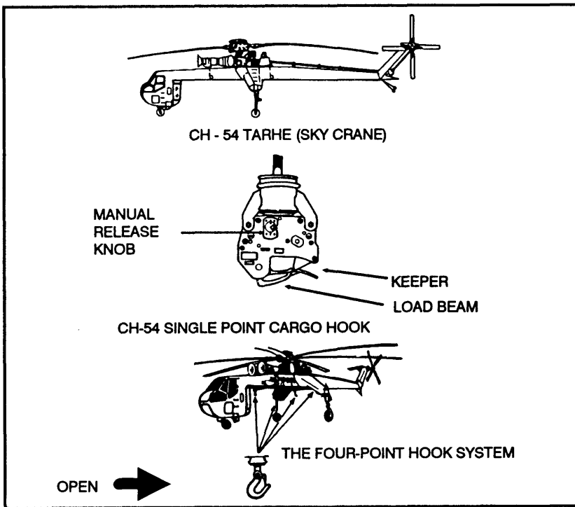
Figure 5-10. CH-54 Skycrane and its cargo hooks.
