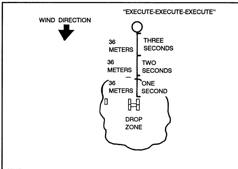
Figure 6-8. Army VIRS off-set.
