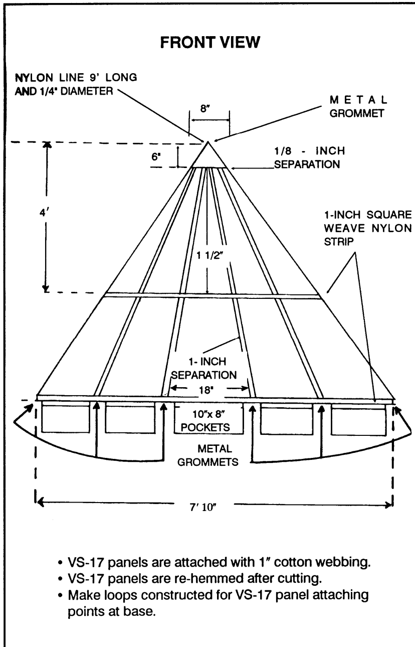
Figure 6-9. Raised angle marker.
