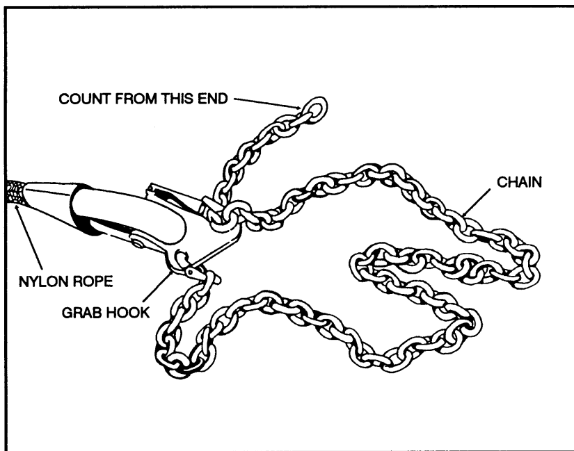
Figure 5-5. Coupling link.
