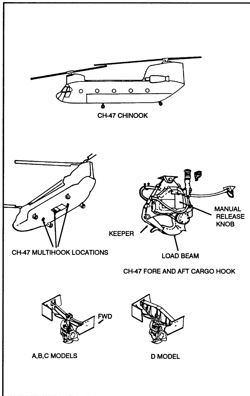
Figure 5-11. CH-47 Chinook and its cargo hooks.
